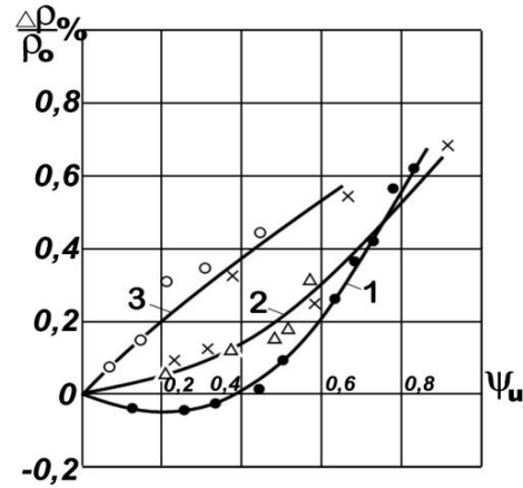
Fig. 3. Dependence of plastic loosening of metals \Delta\rho/\rho_0 on the value of the plasticity resource used: \psi_u : ●, ○ – compression; △ – torsion; × – stretch 1 – EI961 alloy; 2 – VT9 alloy; 3 – EP718 alloy
