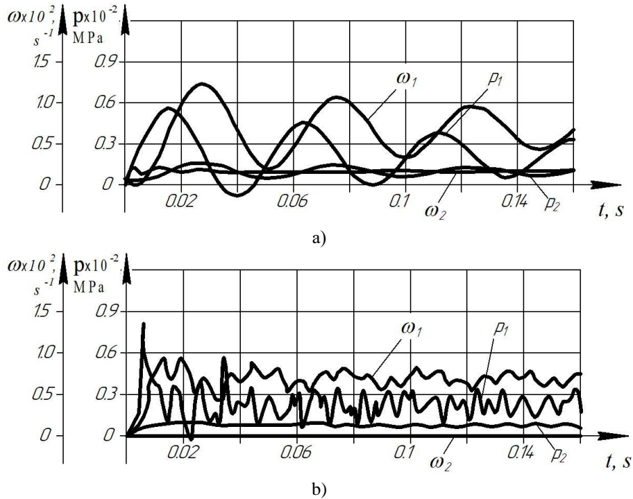
Figure 4. Transient functions of group hydraulic drive operation with two series-connected hydraulic motors with parameters: L = 9 \text{ m} , ( W_1 = 19.5 \cdot 10^{-4} \text{ m}^3 ), in which HM-46 hydraulic oil was used: a) without taking into account wave processes; b) taking into account wave processes.
