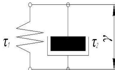
Fig. 4. Rheological model of maize grain germ
