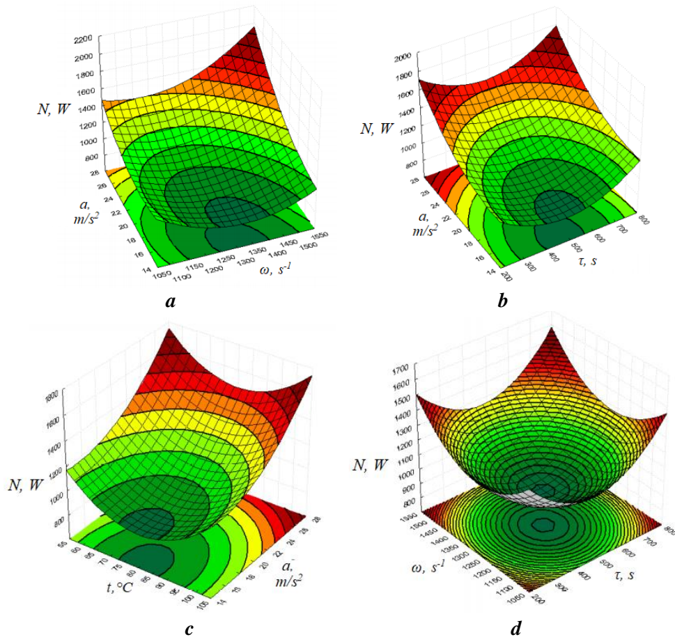
Fig. 2. Surface feedback characterizing energy costs from: a) N_{tot.} = f(a, \omega_{rot}) , b) N_{tot.} = f(a, \tau) ; c) N_{tot.} = f(a, t_{gl}) , d) N_{tot.} = f(\omega_{rots}, \tau)
