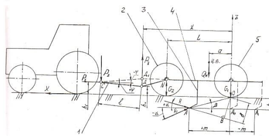
Fig. 1. Calculation scheme of the unit with a trailer:
